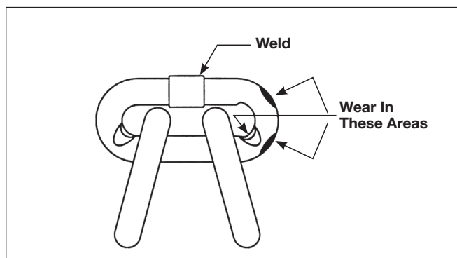
Figure 6 - Chain Inspection
