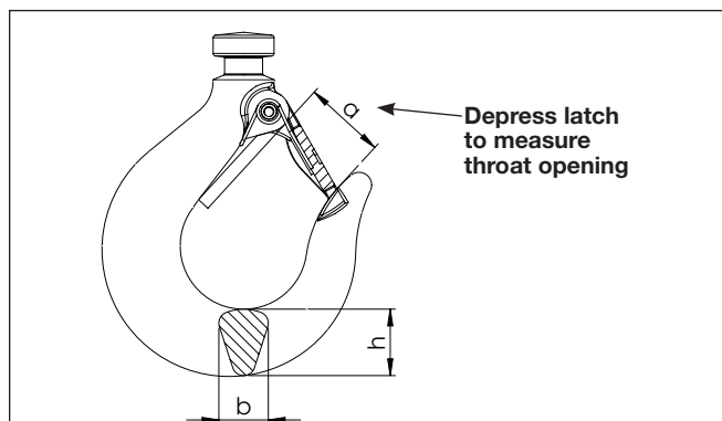
Figure 5 - Hook Inspection
